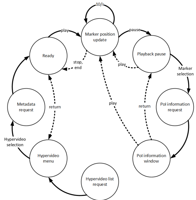
Figure 11. Sequence diagram of the module states. Dotted transitions denote backwards transitions.
