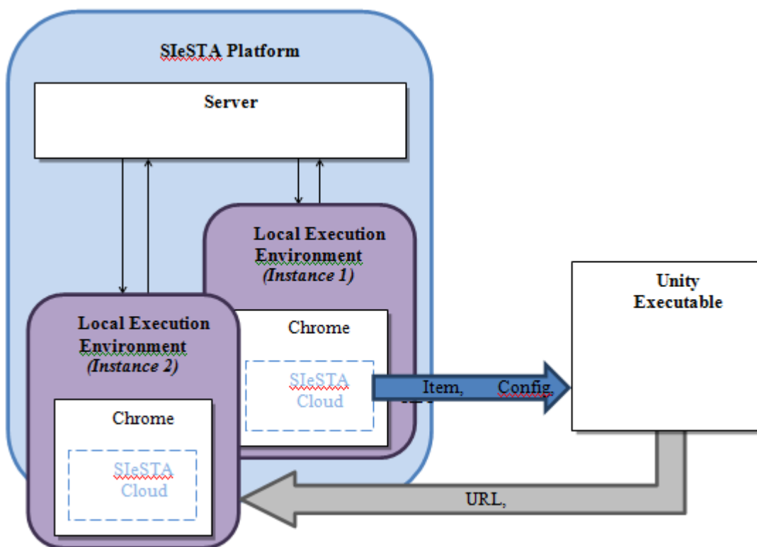
Figure 7. SIESTA-UNITY Communication
