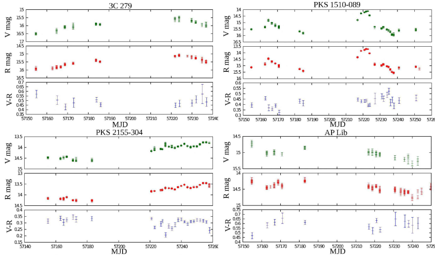
Figure 1. V, R and V-R light curves for 3C 279 ( top left ), PKS1510-089 ( top right ), PKS 2155-304 ( bottom left ) and AP Lib ( bottom right ).
