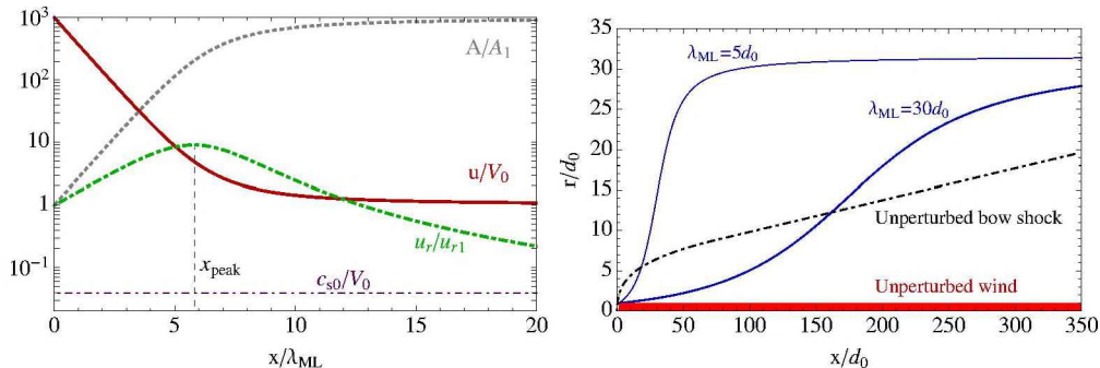
Figure 2. Left: structure of a pulsar wind when mass loading occurs. The various lines represent the wind speed divided by V_0 (solid line), wind cross section (dotted line) and radial expansion speed (dot-dashed line) both normalized to their initial values. The sound speed of the ISM, c_{s0} , also normalized to V_0 , is shown for comparison (thin dot-dashed line). Right: comparison between two mass loaded wind profiles, calculated using \lambda_{\text{ML}} = 5d_0 (thin lines) and \lambda_{\text{ML}} = 30d_0 (thick lines), and the profile of the unperturbed bow shock, calculated using the thin shock approximation (dot-dashed line; Wilkin 1996). The shaded region, with radius r = d_0 , shows the unperturbed pulsar wind, i.e. without the mass loading effect. Adapted from Morlino et al. (2015).
