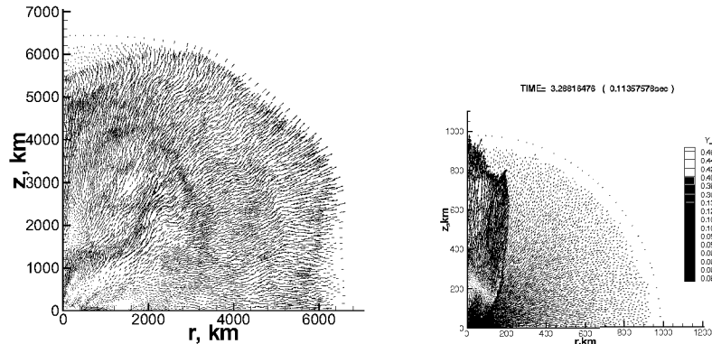
Figure 2. The velocity field (outflow) for the time moment, t = 0.25 s, from Moiseenko et al. (2006, left). Jet formed for the initial uniform field with H_{0z} = 10^9 Gs, E_{\text{rot},0}/E_{\text{grav},0} = 0.8\% . The hatched zone corresponds to the outflowing jet, ejected from deep layers of the star with high neutronization, low Y_e = n_e/n_b , where n_e is the electron concentration, n_b is a total baryon concentration (free and in nuclei, right) . Left panel reproduced from Bisnovatyi-Kogan et al. (2015).
