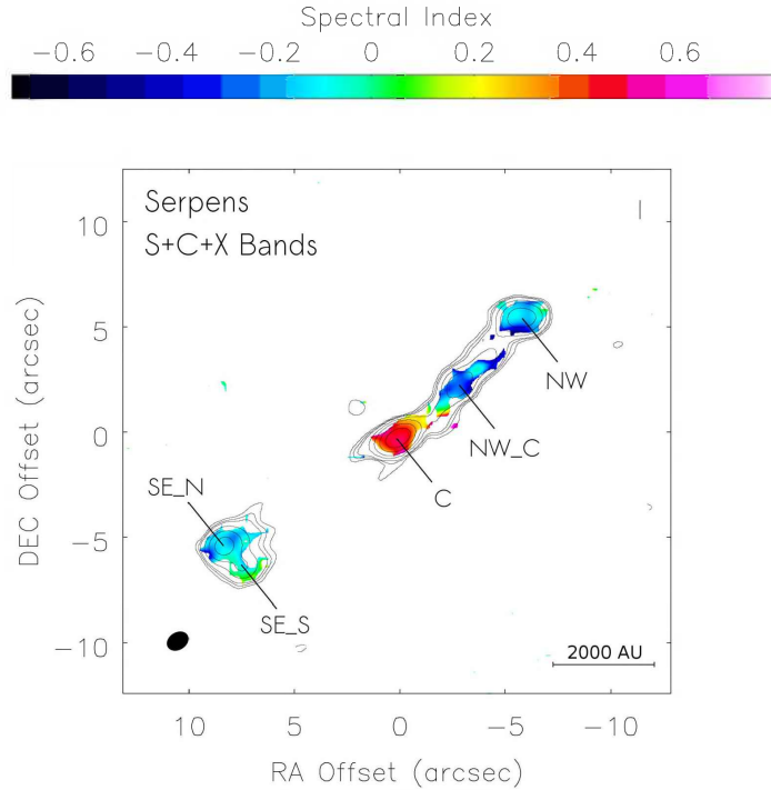
Figure 1. Spatial distribution of spectral indices obtained from multifrequency synthesis cleaning in the frequency range of S, C, and X bands (color scale). The pixels shown are those with an error in the spectral index less than 0.1. This map suggests a clear difference in the emission nature from the powering source and the jet. White contours represent the radio continuum emission with total intensity corresponding to 4, 6, 8, 16, 31, 64, and 128 times the root mean square of the image. The synthesized beam size is 1.07'' \times 0.80'' with a PA of -58^\circ (bottom left). The four components discussed in the paper are labeled. Reproduced from Rodríguez-Kamenetzky et. al (2016).
